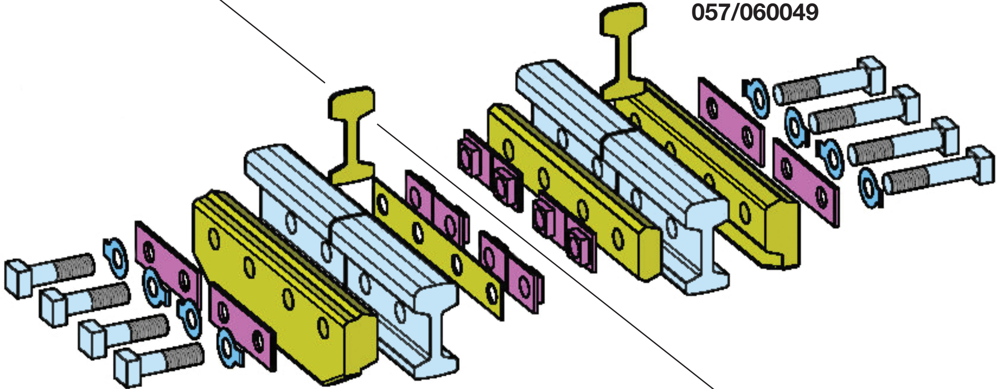
95rBS Check Rail Kit 057/060047
